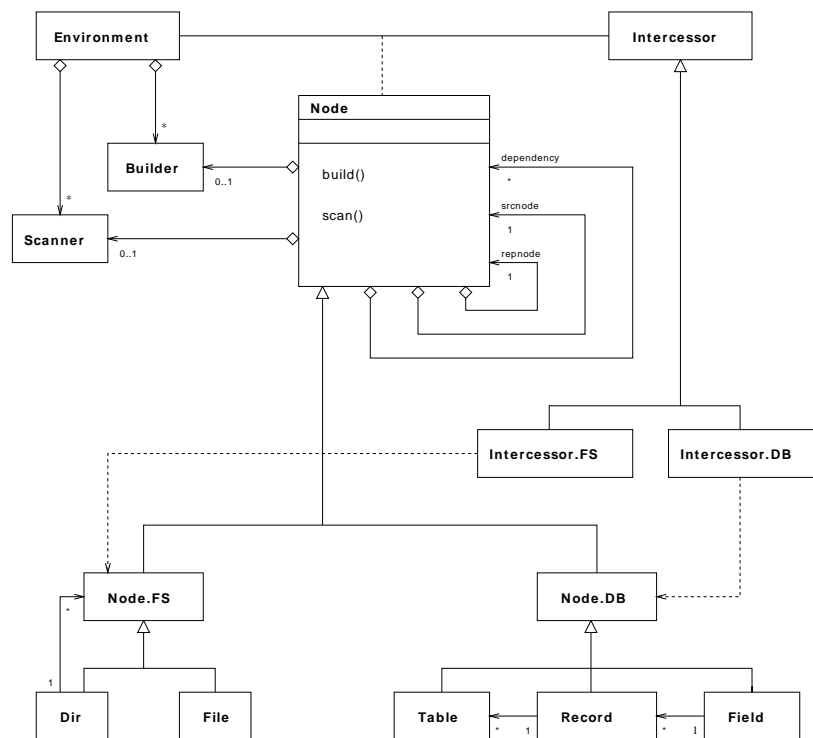
Figure 3.1. SCons Architecture
