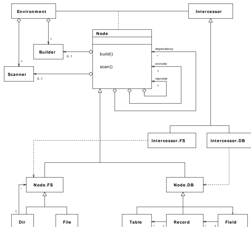
Figure 3.1. SCons Architecture
